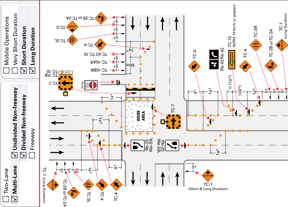
Figure TL-60B Work in Intersection: Two Lanes Closed - Option 2
